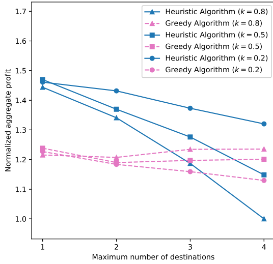
Figure 7. Normalized aggregate profit ( \varrho^r + \rho^r ) for the heuristic and greedy algorithms over random topology with |N| = 25 , K = 4 , \eta^r = 1 , and L is set to the maximum hop distance between any pair of nodes.
