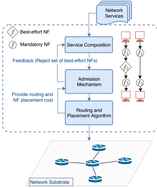
Figure 1. The joint all-or-nothing/all-or-something admission mechanism and online JCRP framework.
