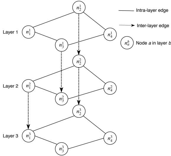
Figure 3. The auxiliary network transformation for the problem input in Fig. 2.
