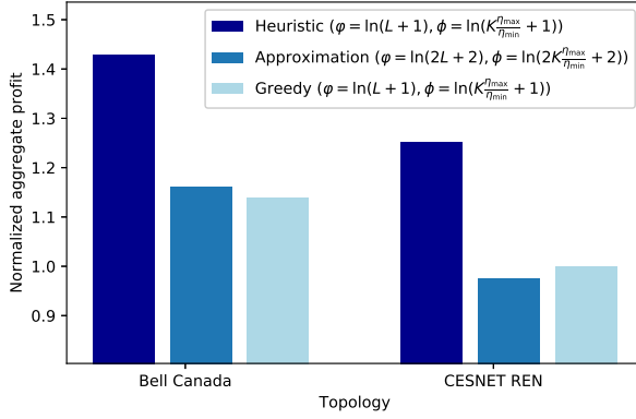
Figure 6. Normalized aggregate profit ( \varrho^r + \rho^r ) for the three algorithms for two real topologies, namely Bell Canada and CESNET REN, with K = 5 and L = 13 and 6 , respectively.
